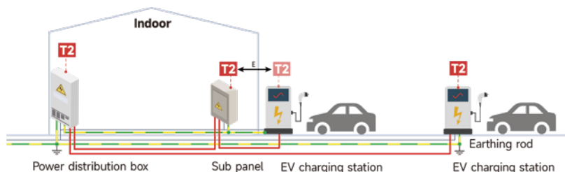
SCENE 4 SPD for outdoor EVSE – without lightning protection system (LPS)
