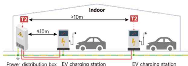
SCENE 2 SPD for indoor EVSE – without lightning protection system (LPS)
