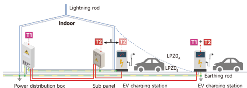
SCENE 3 SPD for outdoor EVSE – with lightning protection system (LPS)
